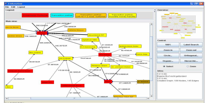
Fig.: Siron® LinkAnalysis – cash flows
